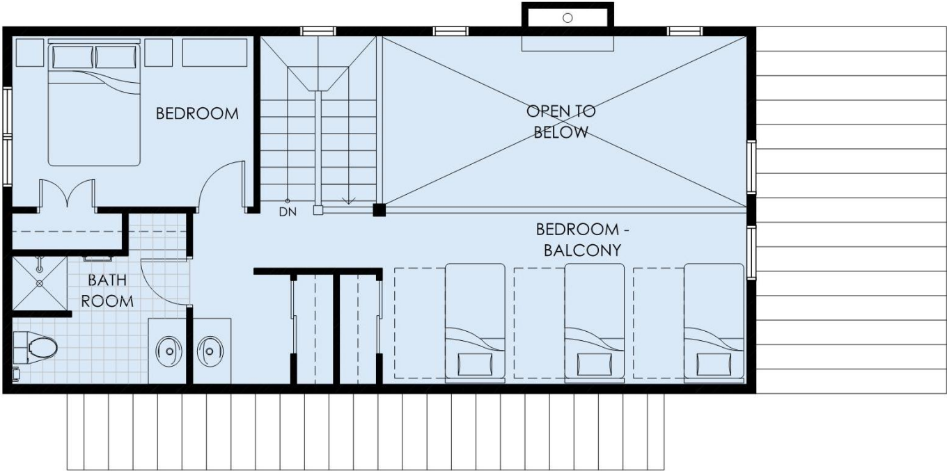
SECOND FLOOR UNIT 611
